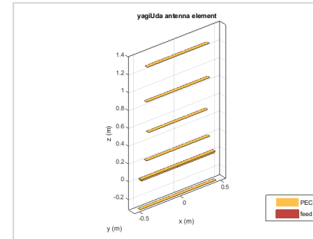
Parameterized antenna geometry
