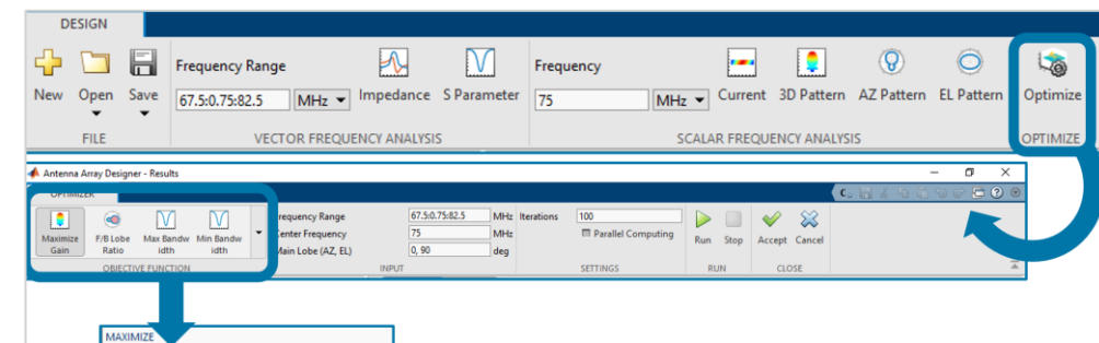
App workflow: choose objective, run, review, accept
